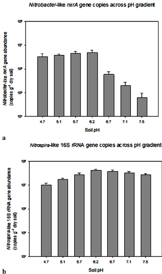
Fig. 1. Effect of pH effects on abundances of Nitrobacter nxrA (a) and Nitrospira (b) gene abundance ( \text{g}^{-1} dry soil).
